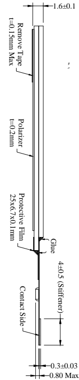
(Reference Mechanical Design)
