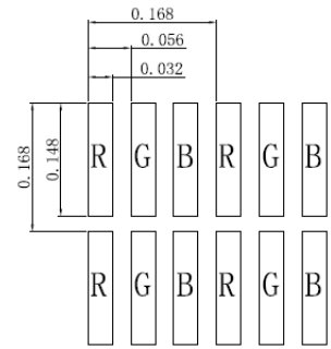
Detail A (30:1)
