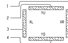
TP pins assignment
